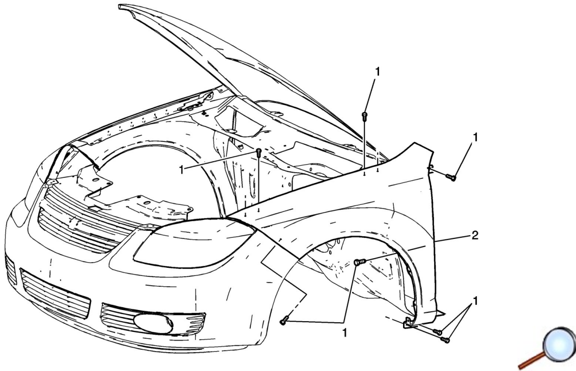
Front Fender Replacement
